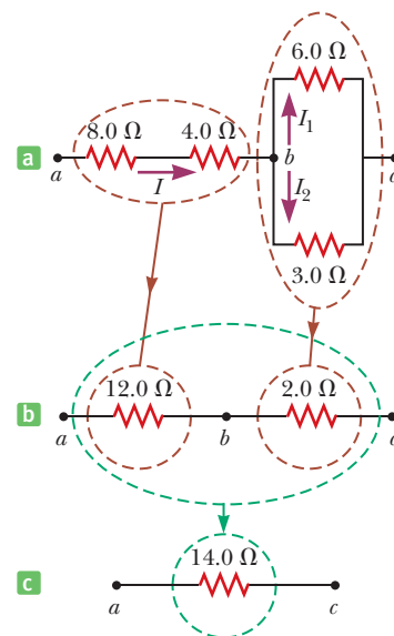
Figure 18.11 (Example 18.3) The four resistors shown in (a) can be reduced in steps to an equivalent 14-Ω resistor.
