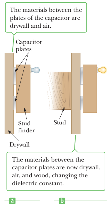
Figure 16.28 (Applying Physics 16.2) A stud finder produces an electric field that is affected by the dielectric constant of the materials placed in its field. When the device moves across a stud, the change in dielectric constant activates a signal light.
