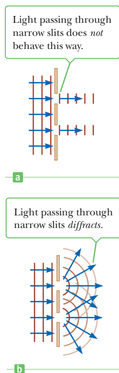
Figure 24.13 (a) If light did not spread out after passing through the slits, no interference would occur. (b) The light from the two slits overlaps as it spreads out, filling the expected shadowed regions with light and producing interference fringes.
