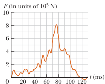
Figure 6.5 Force on a car versus time for a typical collision.
