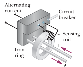
Figure 20.11 Essential components of a ground fault interrupter (contents of the gray box in Fig. 20.12a, page 696). In newer homes such devices are built directly into wall outlets. The purpose of the sensing coil and circuit breaker is to cut off the current before damage is done.
