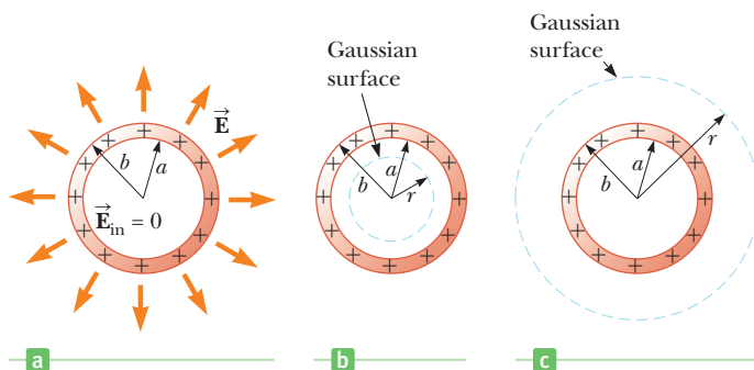
Figure 15.29 (Example 15.7) (a) The electric field inside a uniformly charged spherical shell is zero. It is also zero for the conducting material in the region a < r < b . The field outside is the same as that of a point charge having a total charge Q located at the center of the shell. (b) The construction of a Gaussian surface for calculating the electric field inside a spherical shell. (c) The construction of a Gaussian surface for calculating the electric field outside a spherical shell.
