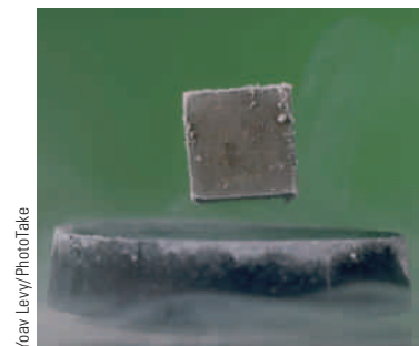
Figure 17.12 A small permanent magnet floats freely above a nitrogen-cooled ceramic superconductor. The superconductor has zero resistance and expels any magnetic field from inside the superconductor by creating a mirror image of the magnetic poles of the permanent magnet. This “Meissner effect” results in magnetic levitation of the permanent magnet.
