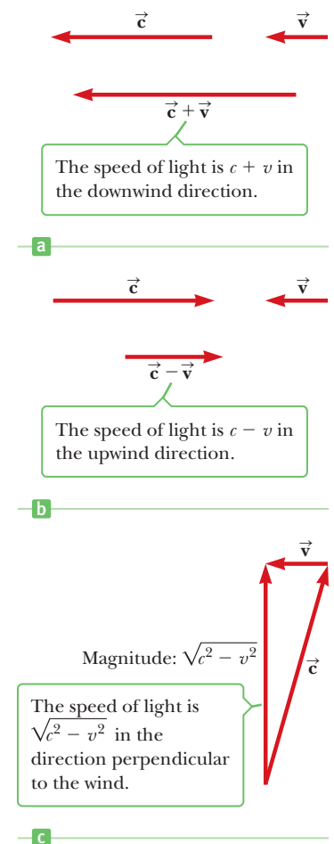
Figure 26.3 If the speed of the ether wind relative to Earth is v and c is the speed of light relative to the ether, the speed of light relative to Earth is (a) c + v in the downwind direction, (b) c - v in the upwind direction, and (c) \sqrt{c^2 - v^2} in the direction perpendicular to the wind. The Michelson–Morley experiment, however, disproved the ether wind hypothesis, leading to Einstein's postulate that the speed of light in vacuum has the same value regardless of the motion of an inertial observer.
