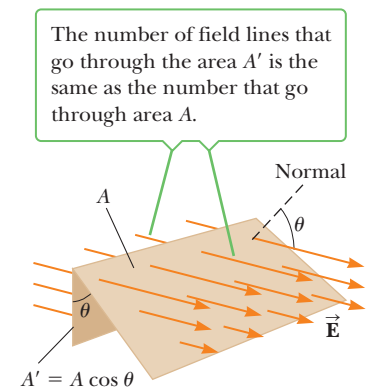
Figure 15.25 Field lines for a uniform electric field through an area A that is at an angle of (90^\circ - \theta) to the field.
