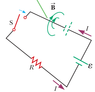
Figure 20.23 After the switch in the circuit is closed, the current produces its own magnetic flux through the loop. An opposing emf is therefore induced, meaning the current relatively slowly increases toward its maximum value rather than jumping to that value right away. The battery with the dashed lines is a symbol for the self-induced emf.
