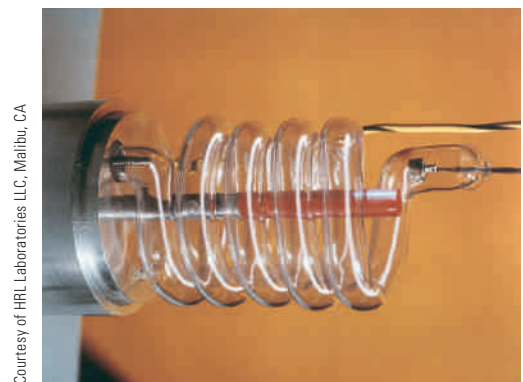
Figure 28.21 (a) Steps in the production of a laser beam. (b) Photograph of the first ruby laser, showing the flash lamp surrounding the ruby rod.
