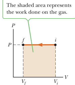
Figure 12.3 The PV diagram for a gas being compressed at constant pressure.
