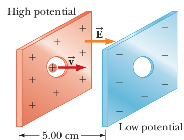
Figure 16.4 (Example 16.3) A proton enters a cavity and accelerates from one charged plate toward the other in an electric field \vec{E} .
