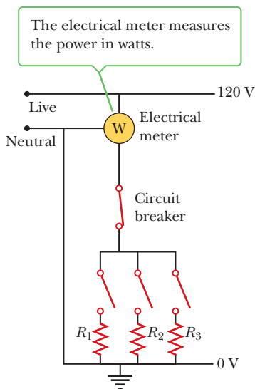
Figure 18.20 A wiring diagram for a household circuit. The resistances R_1 , R_2 , and R_3 represent appliances or other electrical devices that operate at an applied voltage of 120 V.
