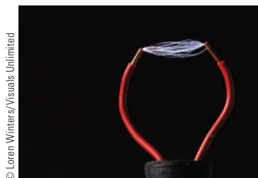
Figure 16.25 Dielectric breakdown in air. Sparks are produced when a large alternating voltage is applied across the wires by a high-voltage induction coil power supply.
