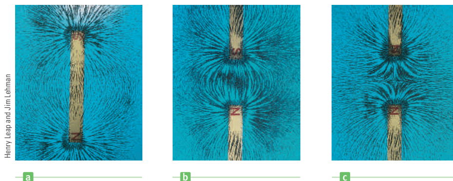
Figure 19.3 (a) The magnetic field pattern of a bar magnet, as displayed with iron filings on a sheet of paper. (b) The magnetic field pattern between unlike poles of two bar magnets, as displayed with iron filings. (c) The magnetic field pattern between two like poles.
