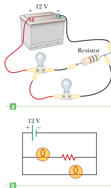
Figure 16.17 (a) A real circuit and (b) its equivalent circuit diagram.
