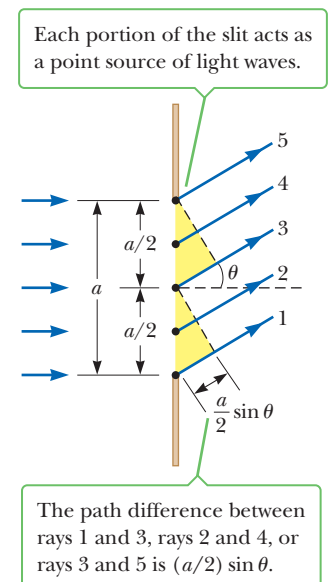
Figure 24.17 Diffraction of light by a narrow slit of width a . (This drawing is not to scale, and the waves are assumed to converge at a distant point.)
