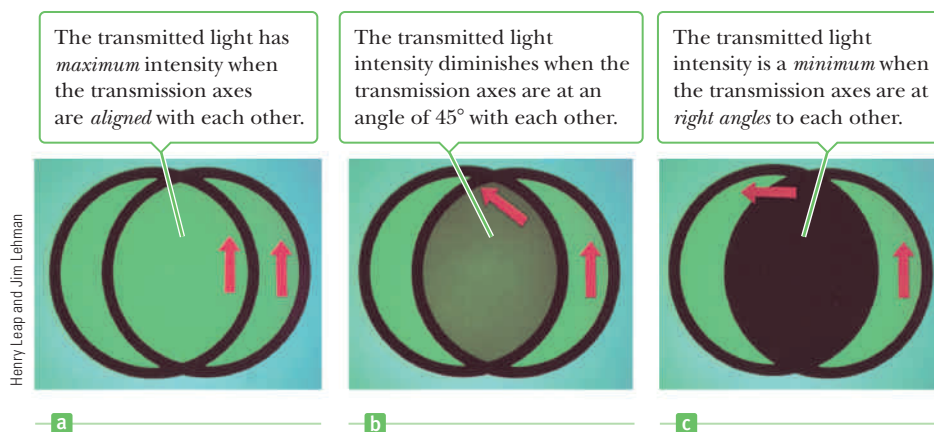
Figure 24.27 The intensity of light transmitted through two polarizers depends on the relative orientations of their transmission axes.
