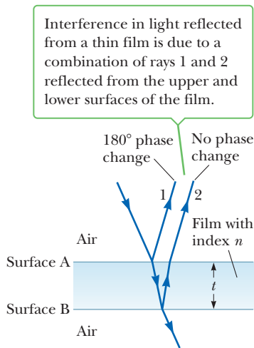
Figure 24.7 Light passes through a thin film.
