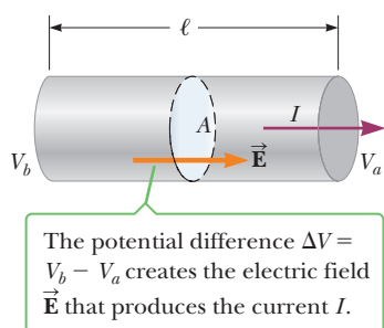
Figure 17.7 A uniform conductor of length \ell and cross-sectional area A . The current I is proportional to the potential difference or, equivalently, to the electric field and length.
