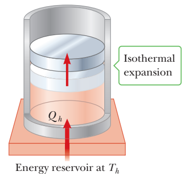
Figure 12.7 The gas in the cylinder expands isothermally while in contact with a reservoir at temperature T_h .
