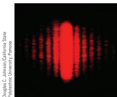
Figure 24.14 The diffraction pattern that appears on a screen when light passes through a narrow vertical slit. The pattern consists of a broad central band and a series of less intense and narrower side bands.
