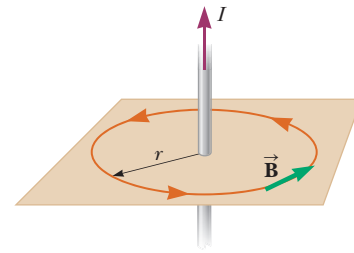
Figure 19.26 A closed, circular path of radius r around a long, straight, current-carrying wire is used to calculate the magnetic field set up by the wire.
