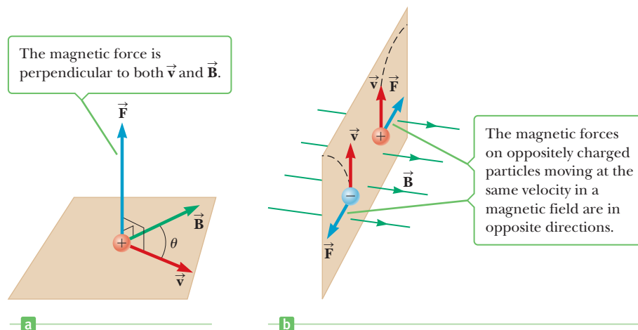
Figure 19.6 (a) The direction of the magnetic force \vec{F} acting on a charged particle moving with a velocity \vec{v} in the presence of a magnetic field \vec{B} . (b) Magnetic forces on positive and negative charges. The dashed lines show the paths of the particles, which are investigated in Section 19.6.
