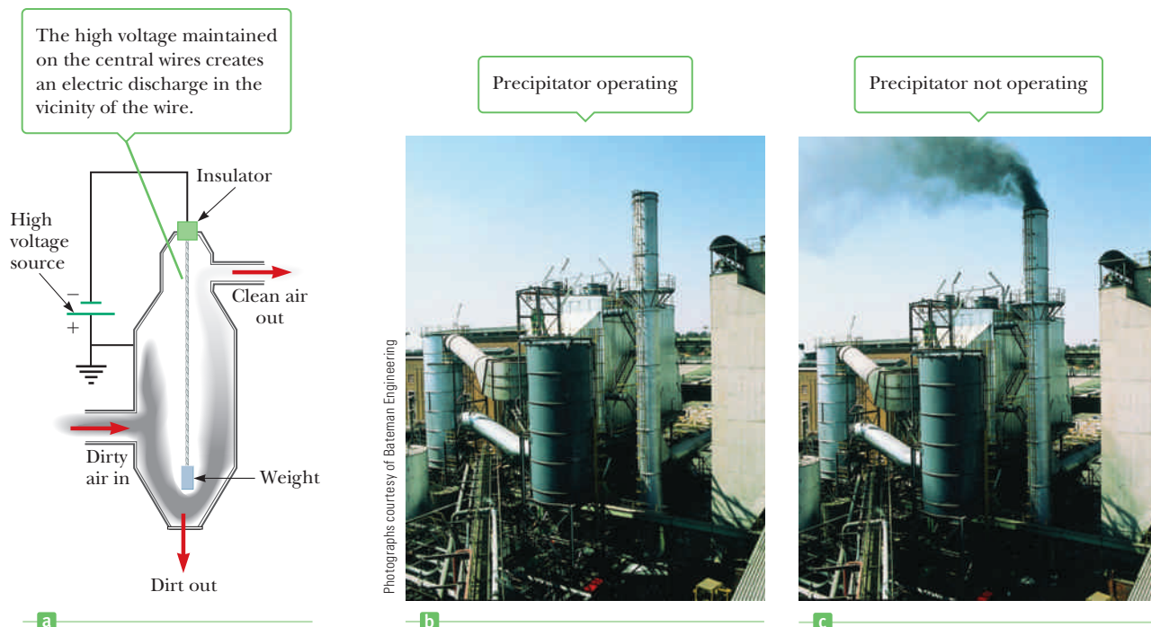
Figure 16.12 (a) A schematic diagram of an electrostatic precipitator. Compare the air pollution when the precipitator is (b) operating and (c) turned off.
