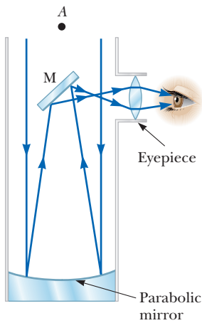
Figure 25.9 A reflecting telescope with a Newtonian focus.
