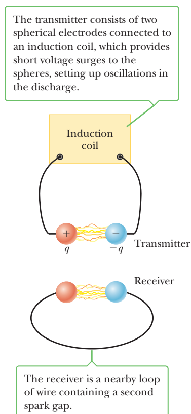
Figure 21.17 A schematic diagram of Hertz's apparatus for generating and detecting electromagnetic waves.
