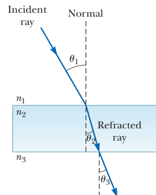
Figure 22.11 (Example 22.2) Refraction of light by glass.
