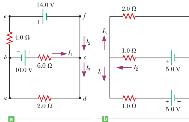
Figure 18.15 (a) (Example 18.5) (b) (Exercise 18.5)
