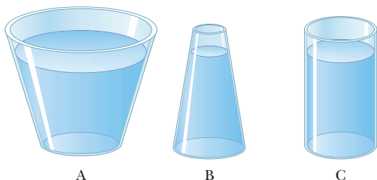
Figure MCQ9.10
