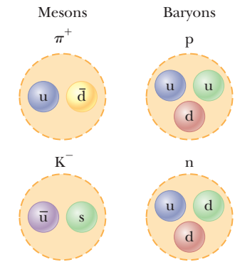
Active Figure 30.8 Quark compositions of two mesons and two baryons. Note that the mesons on the left contain two quarks and that the baryons on the right contain three quarks.
