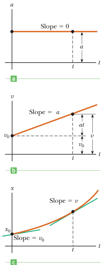
Active Figure 2.15
