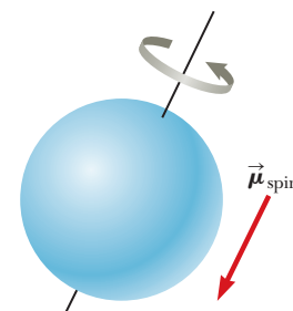
Figure 19.37 Classical model of a spinning electron.
