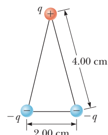
Figure P16.17
