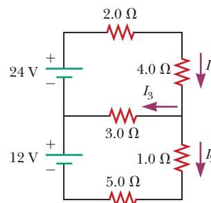
Figure P18.25
