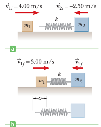
Figure 6.14 (Example 6.7)
