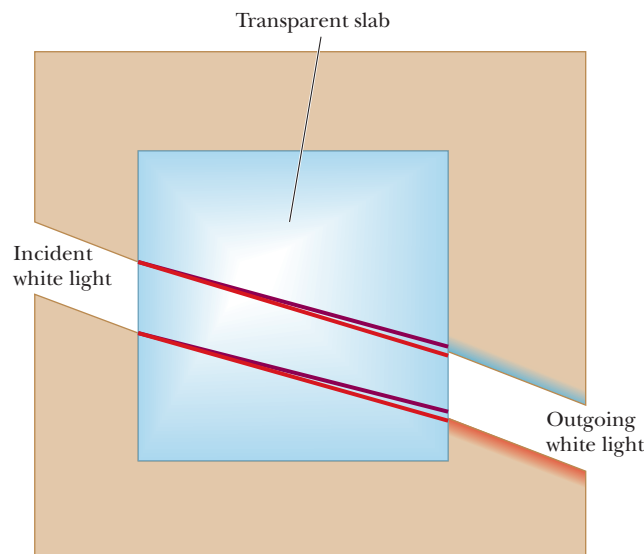
Figure 22.17 (Applying Physics 22.3)
