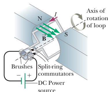
Active Figure 19.17
