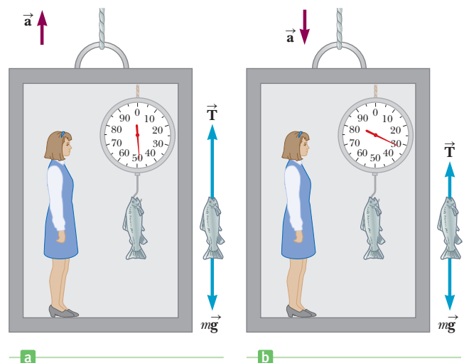
Figure 4.19 (Example 4.10)
