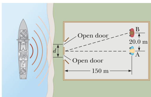
Figure P24.11
