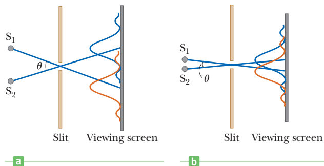
Two point sources far from a narrow slit each produce a diffraction pattern. (a) The sources are separated by a large angle. (b) The sources are separated by a small angle.
