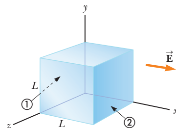
Figure 15.26 (Example 15.6) A hypothetical surface in the shape of a cube in a uniform electric field parallel to the x -axis. The net flux through the surface is zero when the net charge inside the cube is zero.
