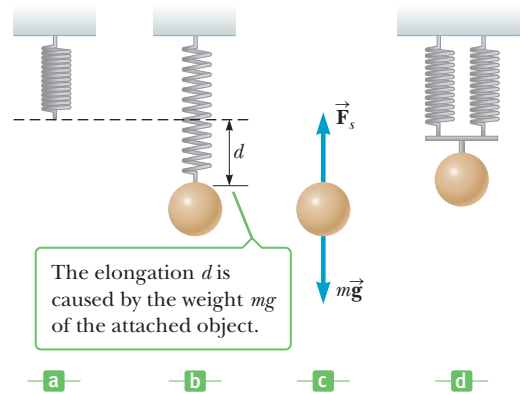
Figure 13.2 (Example 13.2) (a)–(c) Determining the spring constant. Because the upward spring force balances the weight when the system is in equilibrium, it follows that k = mg/d . (d) A system involving two springs in parallel.
