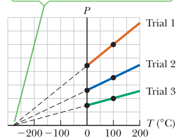
Figure 10.5 Pressure versus temperature for experimental trials in which gases have different pressures in a constant-volume gas thermometer.
