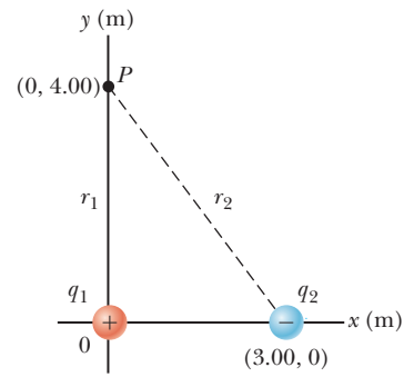
Figure 16.8 (Example 16.4) The electric potential at point P due to the point charges q_1 and q_2 is the algebraic sum of the potentials due to the individual charges.
