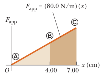
Figure 5.30 (Example 5.15) A graph of the external force required to stretch a spring that obeys Hooke's law versus the elongation of the spring.
