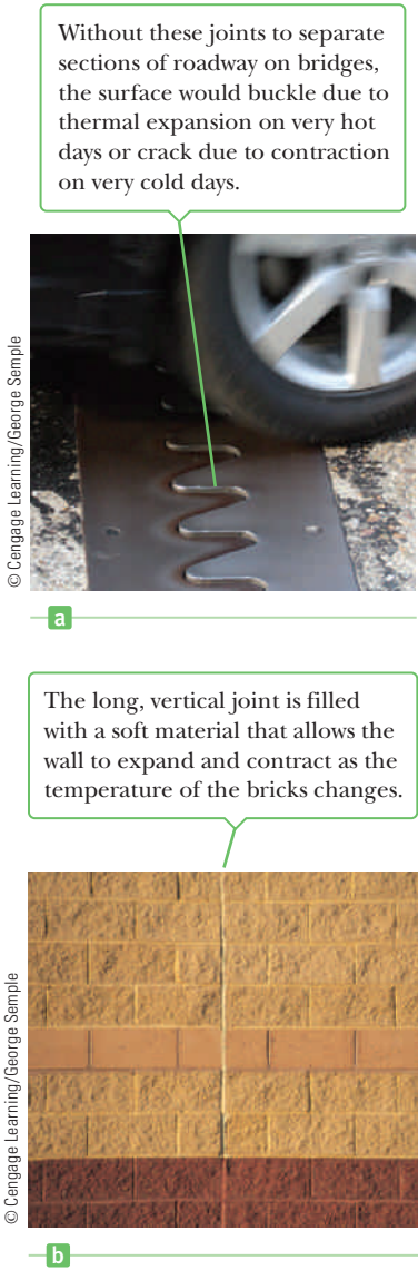
Figure 10.8 Thermal expansion joints in (a) bridges and (b) walls.
