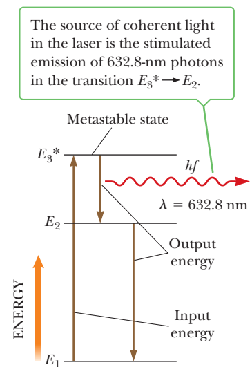
Figure 28.20 Energy level diagram for the neon atom in a helium–neon laser.
