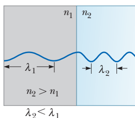
Figure 22.9 A schematic diagram of the reduction in wavelength when light travels from a medium with a low index of refraction to one with a higher index of refraction.
