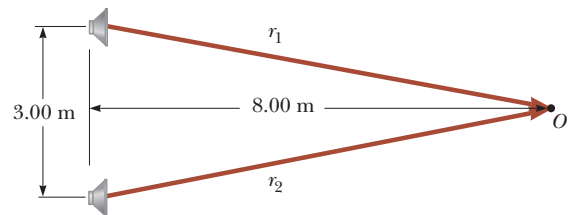
Figure P14.36
