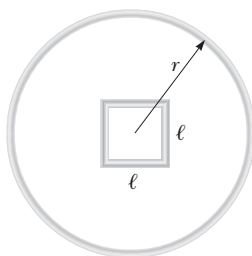
Figure P20.18
