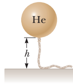
Figure P9.86
