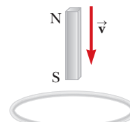
Figure MCQ20.11
