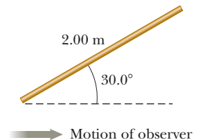
Figure P26.49
