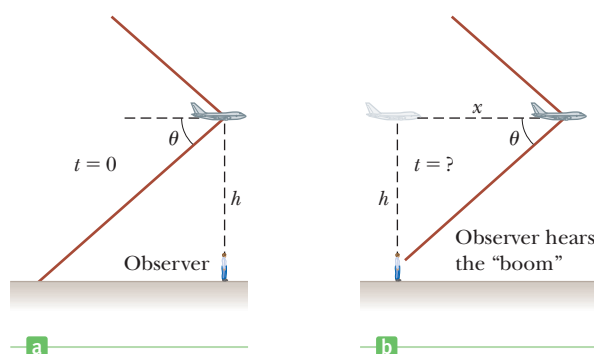
Figure P14.31
