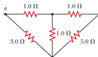
Figure P18.58
