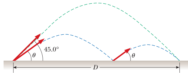
Figure P3.64
