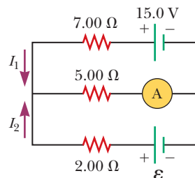
Figure P18.17
