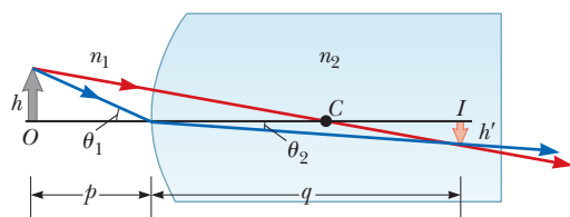
Figure P23.28
