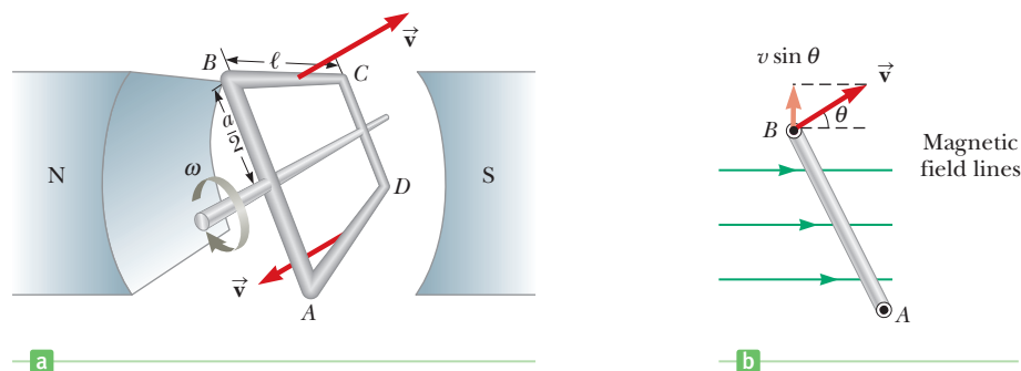
Figure 20.20 (a) A loop rotating at a constant angular velocity in an external magnetic field. The emf induced in the loop varies sinusoidally with time. (b) An edge view of the rotating loop.
