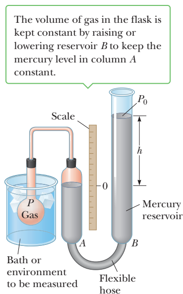
Figure 10.3 A constant-volume gas thermometer measures the pressure of the gas contained in the flask immersed in the bath.
