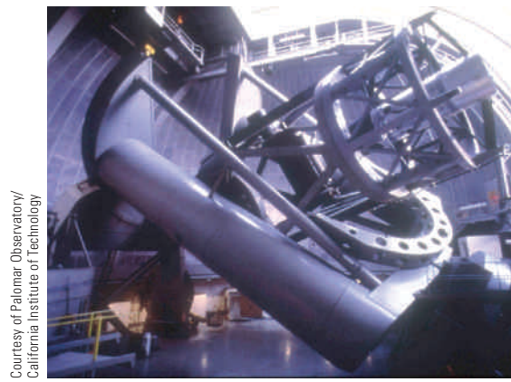
Figure 25.10 The Hale telescope at Mount Palomar Observatory. Just before taking the elevator up to the prime-focus cage, a first-time observer is always told, “Good viewing! And, if you should fall, try to miss the mirror.”
