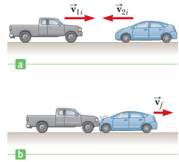
Figure 6.11 (Example 6.4)
