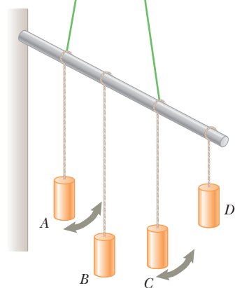
Figure 14.21 A demonstration of resonance.
