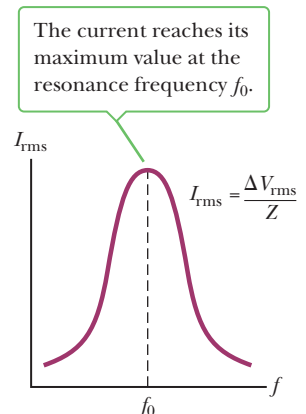
Active Figure 21.13
