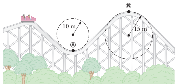
Figure P7.32
