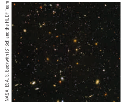
Figure 1.3 In this deep-space photograph, there are few stars—just galaxies without end.
