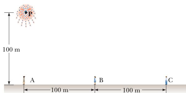
Figure P14.22
