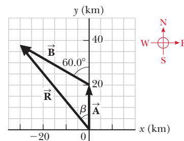
Figure 3.6 (Example 3.1) A graphical method for finding the resultant displacement vector \vec{R} = \vec{A} + \vec{B} .
