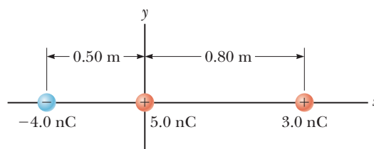
Figure P15.51
