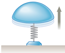
Figure P13.11
