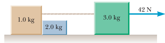
Figure P4.29
