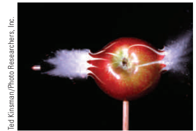
Figure 6.2 An apple being pierced by a 30-caliber bullet traveling at a supersonic speed of 900 m/s. This collision was photographed with a microflash stroboscope using an exposure time of 0.33 \mu\text{s} . Shortly after the photograph was taken, the apple disintegrated completely. Note that the points of entry and exit of the bullet are visually explosive.
