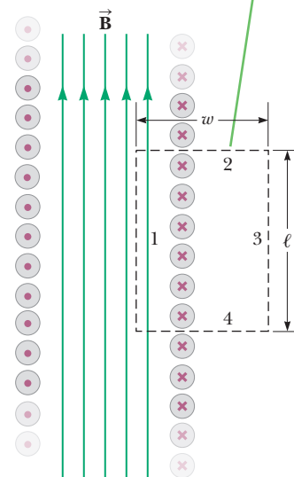
Figure 19.36 A cross-sectional view of a tightly wound solenoid. If the solenoid is long relative to its radius, we can assume the magnetic field inside is uniform and the field outside is zero.
