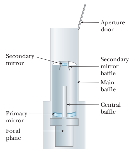
Figure 25.11 A schematic of the Hubble Space Telescope.
