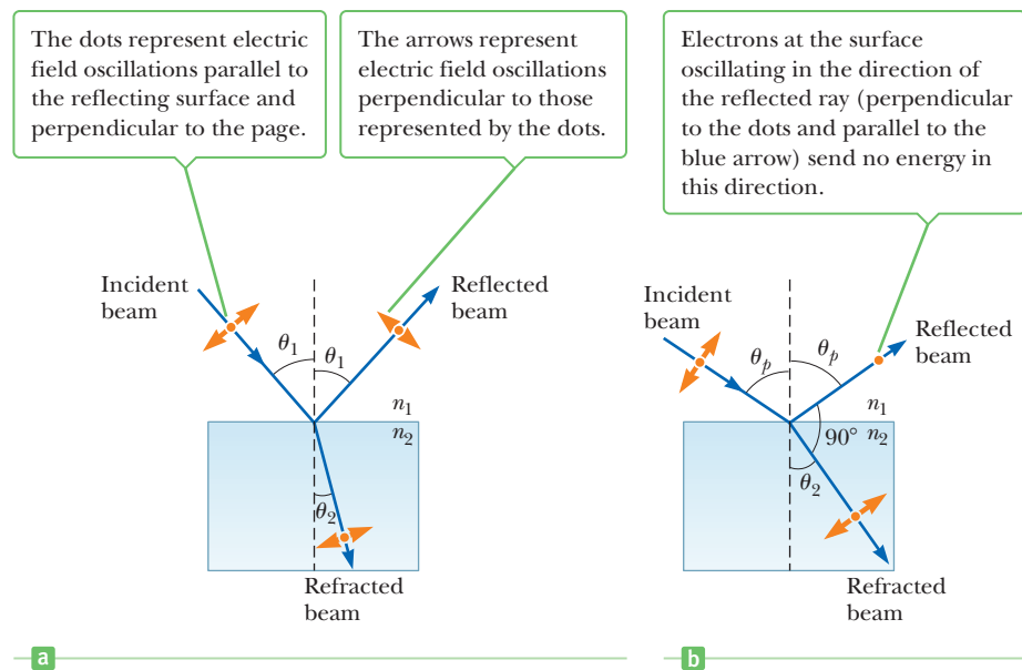
Figure 24.28 (a) When unpolarized light is incident on a reflecting surface, the reflected and refracted beams are partially polarized. (b) The reflected beam is completely polarized when the angle of incidence equals the polarizing angle \theta_p , satisfying the equation n = \tan \theta_p .
