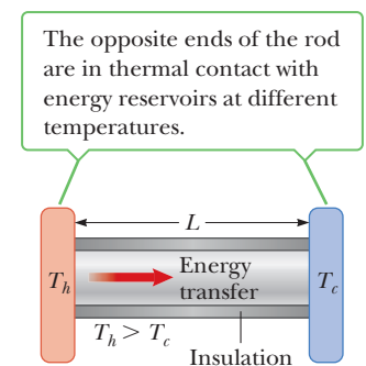
Figure 11.6 Conduction of energy through a uniform, insulated rod of length L .
