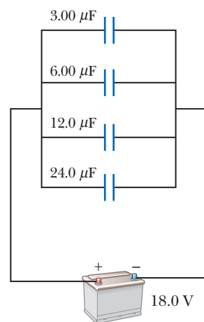
Figure 16.19 (Example 16.7) Four capacitors connected in parallel.
