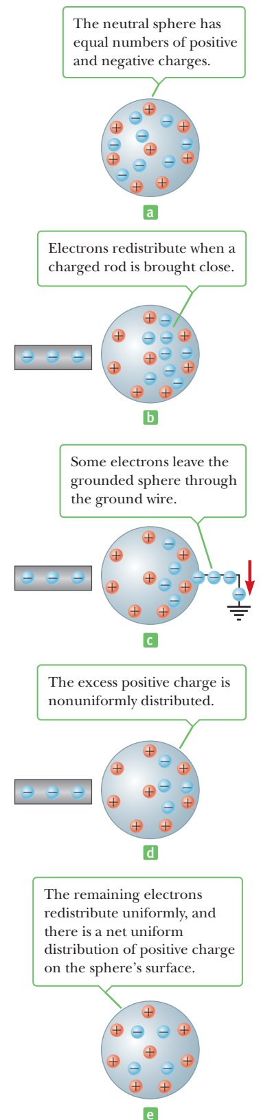
Figure 15.4 Charging a metallic object by induction. (a) A neutral metallic sphere. (b) A charged rubber rod is placed near the sphere. (c) The sphere is grounded. (d) The ground connection is removed. (e) The rod is removed.
