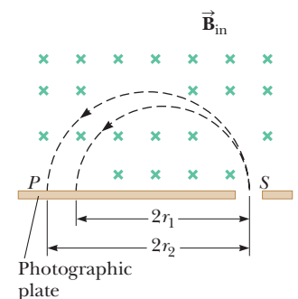
Figure 19.22 (Example 19.6) Two isotopes leave the slit at point S and travel in different circular paths before striking a photographic plate at P.
