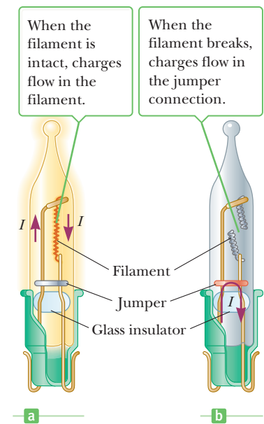
Figure 18.3 (Applying Physics 18.1) (a) Schematic diagram of a modern “miniature” holiday lightbulb, with a jumper connection to provide a current path if the filament breaks. (b) A holiday lightbulb with a broken filament.
