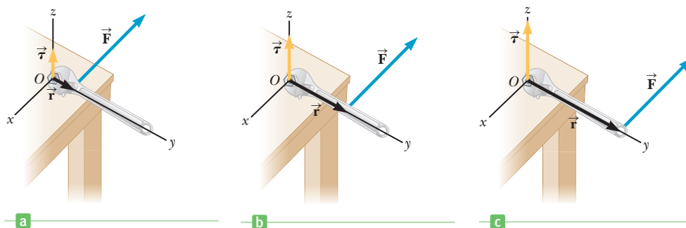
Active Figure 8.2 As the force is applied farther out along the wrench, the magnitude of the torque increases.
