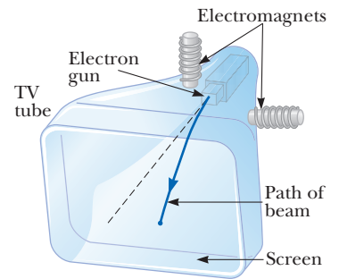
Figure 19.34 Electromagnets are used to deflect electrons to desired positions on the screen of a television tube.
