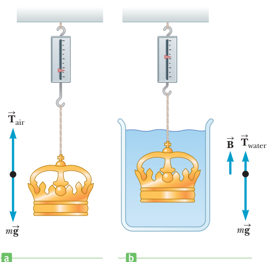
Figure 9.24 (Example 9.8) (a) When the crown is suspended in air, the scale reads T_{\text{air}} = mg , the crown's true weight. (b) When the crown is immersed in water, the buoyant force \vec{B} reduces the scale reading by the magnitude of the buoyant force, T_{\text{water}} = mg - B .
