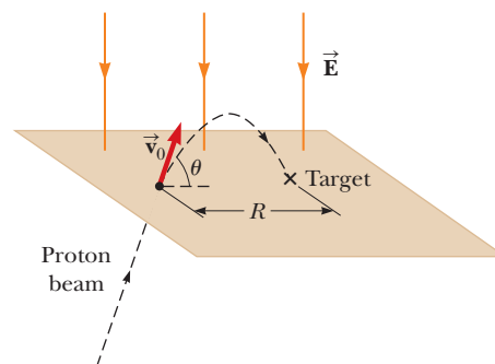
Figure P15.64
