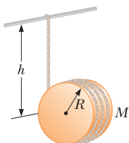
Figure P8.84
