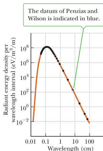
Figure 30.13 Theoretical black-body (rust-colored curve) and measured radiation spectra (black points) of the Big Bang. Most of the data were collected from the Cosmic Background Explorer (COBE) satellite.
