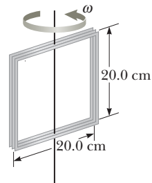
Figure P20.32
