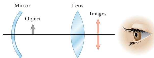
Figure P23.62
