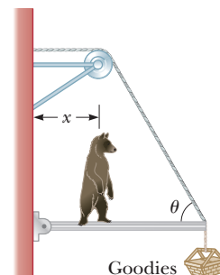
Figure P8.22
