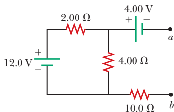
Figure P18.45
