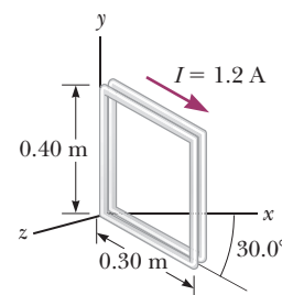
Figure P19.28
