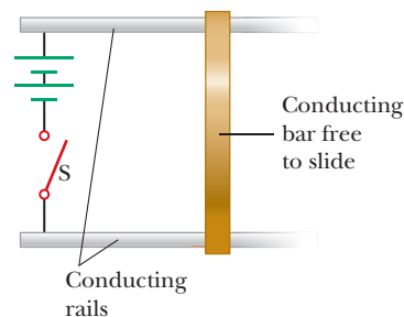
Figure 20.18 (Applying Physics 20.2)
