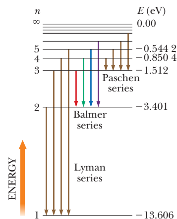
Active Figure 28.8
