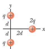
Figure P16.66
