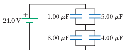
Figure P16.39
