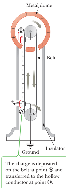
Figure 15.23 A schematic diagram of a Van de Graaff generator. Charge is transferred to the dome by means of a rotating belt.
