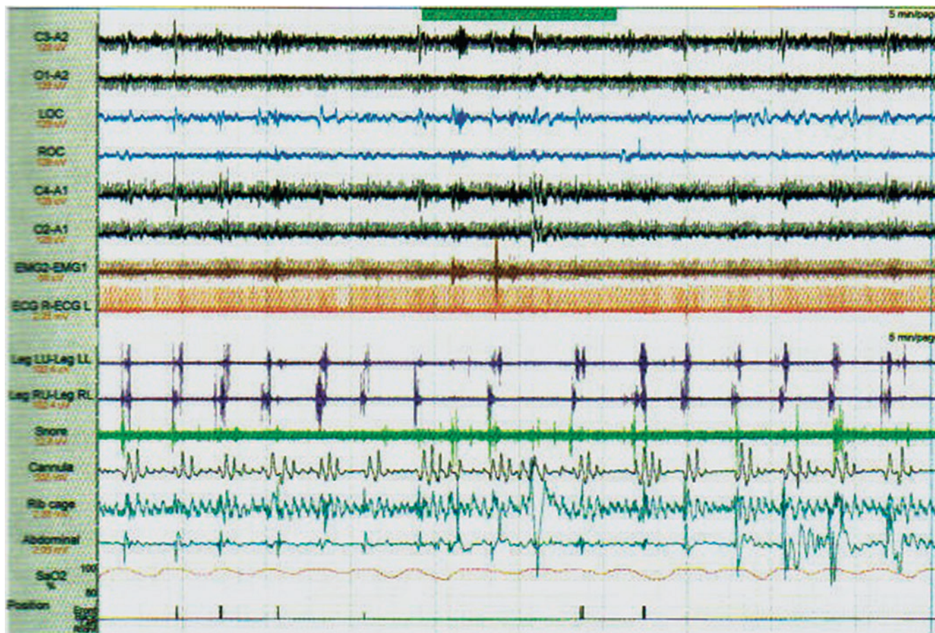
FIG 9.7 A 5-minute epoch of a polysomnogram. C3-A2 , O1-A2 , C4-A1 , and O2-A1 are electroencephalographic leads used to determine sleep stages. LOC and ROC designate eyelid leads at left and right outer canthi, respectively, for recording rapid eye movement. EMG tracing is an electromyogram of the chin used to record jaw movement. ECG tracing is an electrocardiogram that records heart rate and rhythm. Leg LU and Leg RU designate leads for recording leg movements. Snore tracing tracks the subject's snoring. Cannula designates measurement of nasal airflow pressure. Rib cage tracing is a recording of rib cage movement. Abdominal tracing is a recording of abdominal movement. SaO 2 is blood oxygen saturation. Position tracing is a recording of body position. (From Phillips B, Naughton M: Fast facts: obstructive sleep apnea , Oxford, 2004, Health Press Limited.)
